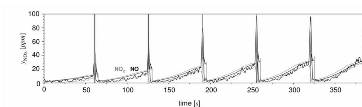
Abb. 15: Simulated cyclic lean-/rich-operation (60s/5s) at 300^\circ C . Catalyst exit concentration of NO and NO_2 versus time compared to measured data for the first six cycles, starting from the completely regenerated catalyst.
