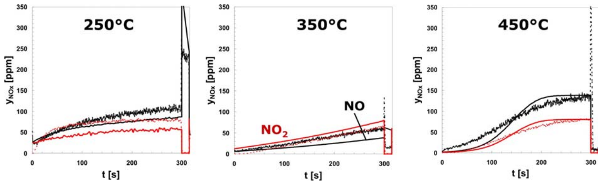
Abb. 20: Lean-/rich-cycle (300s/15s) with the Pt/Ba/Al 2 O 3 -catalyst at different temperatures. Comparison between simulation and experiment.
