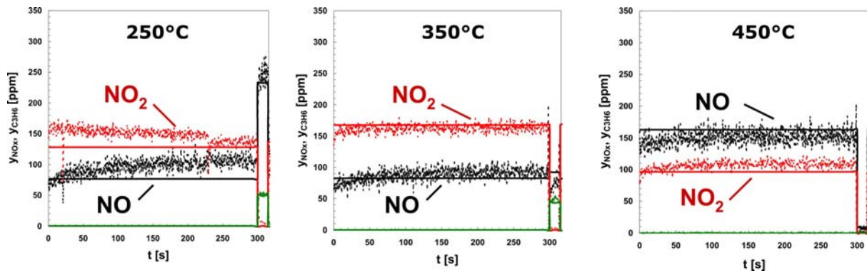
Abb. 17: Lean-/rich-cycle (300s/15s) at different temperatures. Comparison of simulated (line) to measured data (dots).
