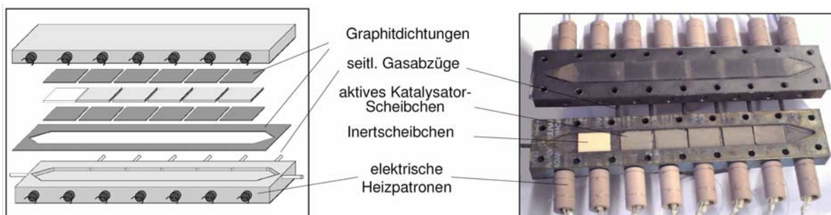
Abb. 2: Monolith slices in the isothermal flat bed reactor.
