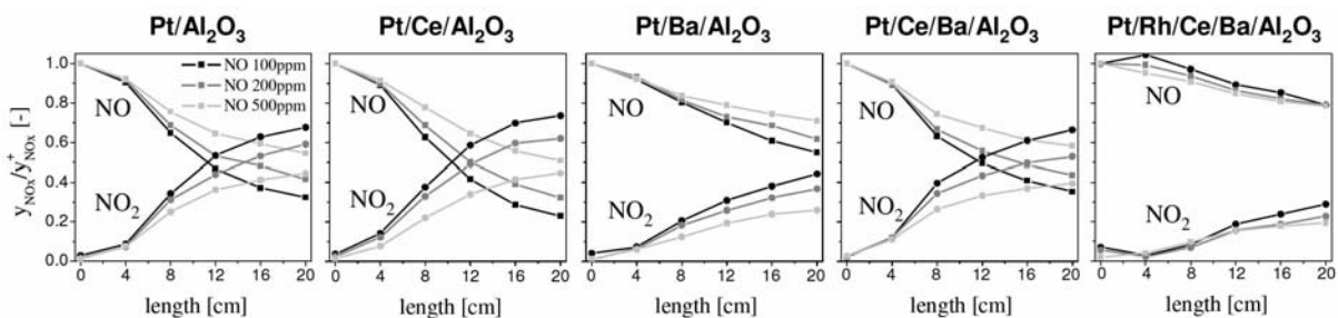
Abb. 3: NO-Oxidation on Pt-containing catalysts under stationary lean conditions at 300°C. NO- and \text{NO}_2 -concentration profiles along the catalyst length, referred to the NO-feed value of 100, 200 and 500ppm.
