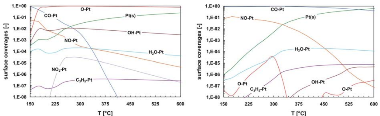
Abb. 16: Calculated surface coverages of Pt in dependence of the temperature. Left: lean phase. Right: rich phase.
