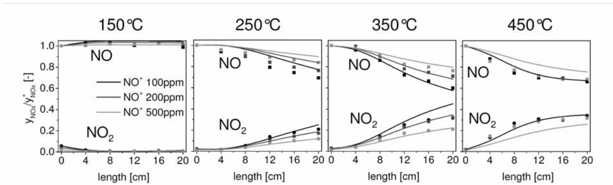
Abb. 12: Simulated NO-oxidation. NO- and \text{NO}_2 -concentration profiles along the catalyst length compared with measurement data in the temperature range from 150°C to 450°C for a NO-feed of 100, 200 and 500ppm, referred to the feed-value.
