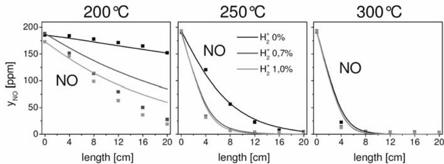
Abb. 13: Simulated NO-reduction. NO-concentration profiles along the catalyst length compared with measurement data in the sensitive temperature range from 200°C to 300°C for a NO-feed of 200ppm and a H 2 -content of 0%, 0.7% and 1.0%.
