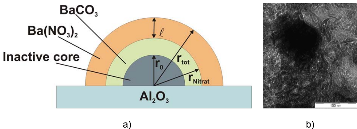
Abb. 18: a) Schematic of the shrinking-core-modell with inactive core. b) TEM-photo of a barium-cluster.
