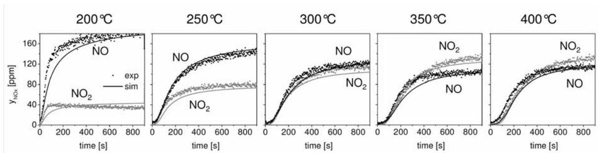
Abb. 14: Simulated NO x -long-time-storage. Catalyst exit concentration of NO and NO 2 versus time compared to measured data for 900s of storage. Temperature range from 200°C to 400°C.
