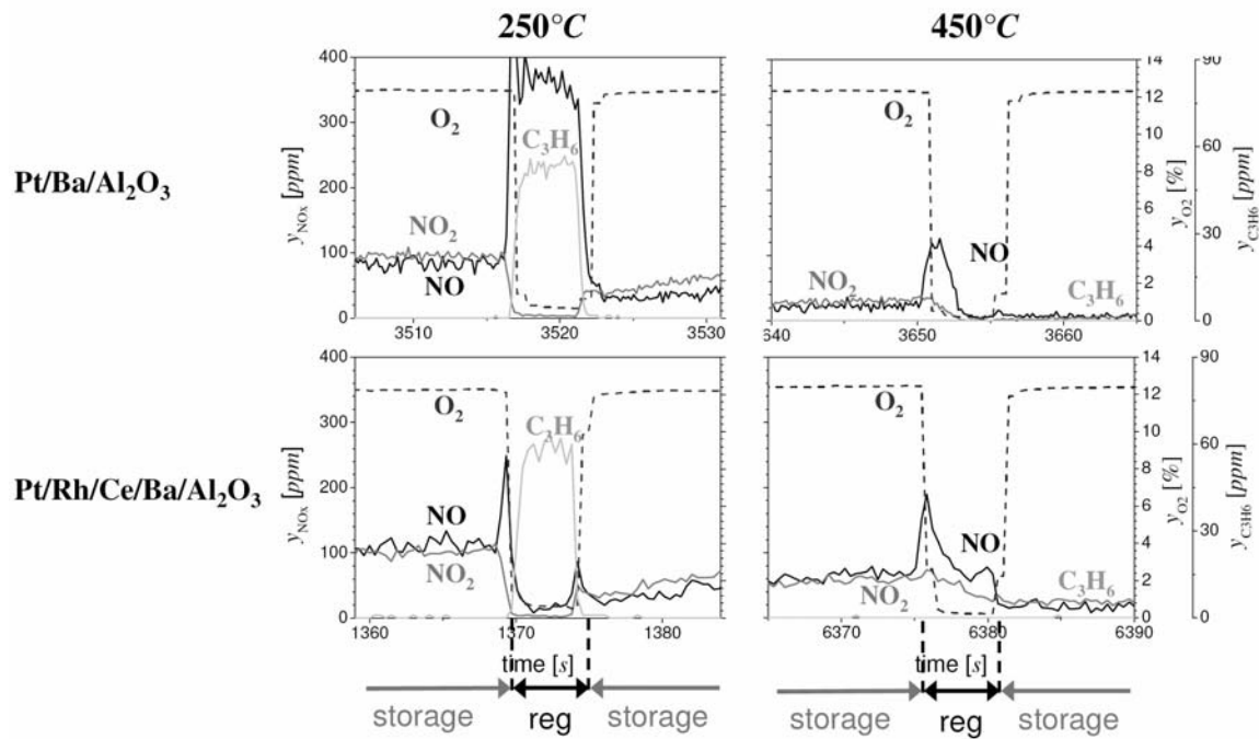
Abb. 9: Catalyst exit concentrations versus time during regeneration, beginning 10s before and ending 10s after the rich phase. Lean-/rich-cycling: 60s/5s. Gas composition according to tab. 2.
