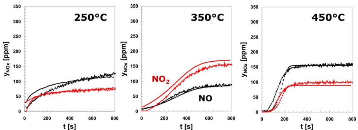
Abb. 19: \text{NO}_x -long-term-storage with the \text{Pt}/\text{Ba}/\text{Al}_2\text{O}_3 -catalyst at different temperatures. Comparison between simulation and experiment.
