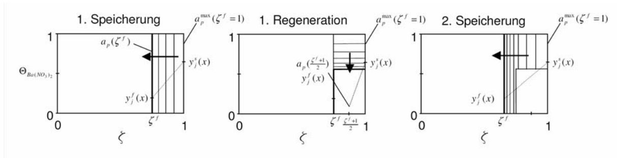
Abb. 11: Schematic of the front proceeding and the nitrate decrease in the storage particle. Plot of the nitrate content in the particle \Theta_{\text{Ba}(\text{NO}_3)_2} versus the dimensionless particle radius \zeta . Left: first storage with a completely regenerated catalyst. Center: first regeneration, uncomplete. Right: second storage with now worse storage performance.
