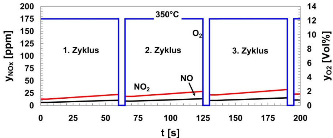
Abb. 21: Simulation of several lean-/rich-cycles (60s/5s) with the Pt/Ba/Al 2 O 3 -catalyst at 350°C.
