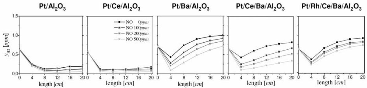
Abb. 5: H_2 -generation on Pt-containing catalysts under stationary rich conditions at 450°C. H_2 -concentration profiles along the catalyst length for a NO-feed of 0, 100, 200 and 500ppm.
