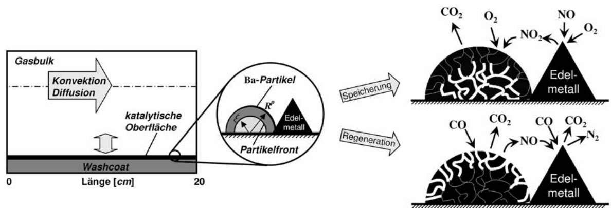
Abb. 10: Model structure of the NSC and schematic of the storage particle.
