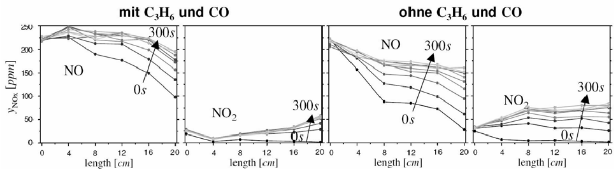
Abb. 6: Concentration-profiles along the catalyst length during \text{NO}_x -storage at the Rh/Ba/ \text{Al}_2\text{O}_3 -sample at 450^\circ\text{C} . Left: with a small amount of CO and \text{C}_3\text{H}_6 in the lean gas (cf. table 2), right: without CO and \text{C}_3\text{H}_6 .
