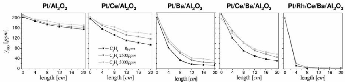
Abb. 4: NO-reduction on Pt-containing catalysts under stationary rich conditions at 300°C. NO-concentration profiles along the catalyst length for a NO-feed of 200ppm and a C 3 H 6 -content of 0, 2500 und 5000ppm.
