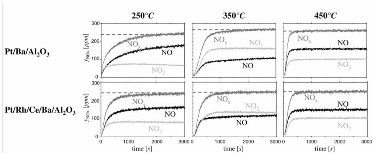
Abb. 7: \text{NO}_x -breakthrough curves during long-time-storage experiments with the \text{Pt/Ba/Al}_2\text{O}_3 - (top) and \text{Pt/Rh/Ce/Ba/Al}_2\text{O}_3 -sample (bottom) at 250^\circ\text{C} , 350^\circ\text{C} und 450^\circ\text{C} . Gas composition according to tab. 2. Dashed line: \text{NO}_x -feed.
