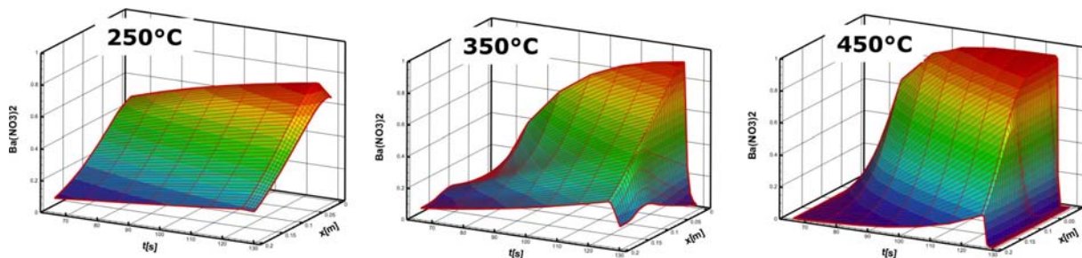
Abb. 22: Calculated surface coverages with \text{Ba}(\text{NO}_3)_2 for the Pt/Ba/Al 2 O 3 -catalyst along the catalyst length (0,2m) in during one lean-/rich-cycle (60s/5s).
